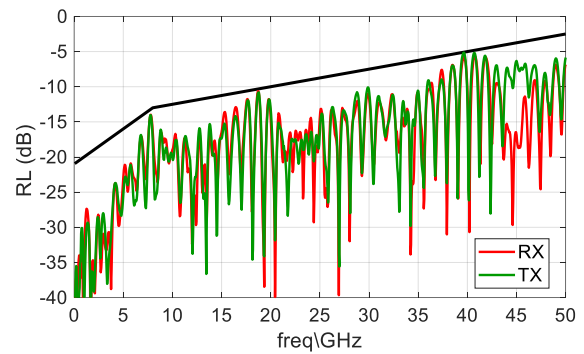
Figure 7: Return Loss – CE-56G-VSR NRZ
