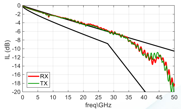
Figure 8: Insertion Loss – CE-56G-VSR NRZ
